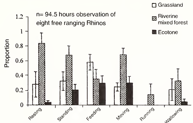
Fig. 5: Proportion of time spent in different activities by wild rhinos in different habitats in the Sauraha area of Chitwan National Park, Nepal
